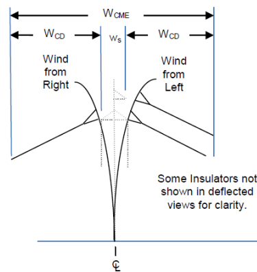
Figure 6.3.4.3-1 – Displaced Conductor Position & Relationship to W_{CME} and w_s
