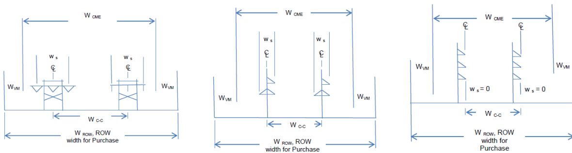
Figure 6.3.4.1-2 – Typical Double Structure ROW
